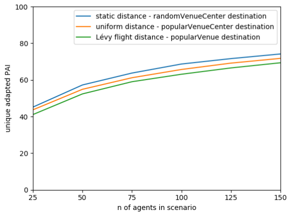
Figure 8: Percentage of crimes covered for best performing scenarios.
